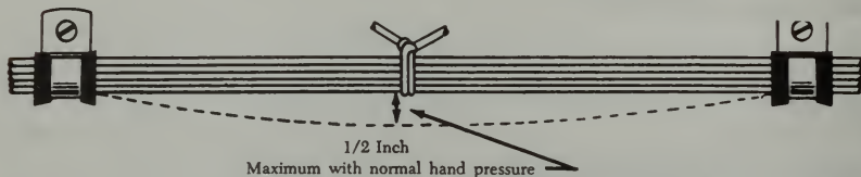
FIGURE 4-91. Slack in wire bundle between supports.
